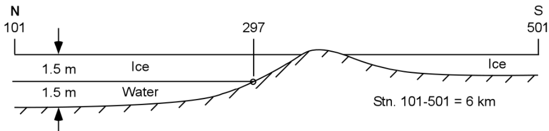
FIG. 1. Schematic diagram of near-surface conditions along the line. Station 297 is the approximate location of the transition from ground-fast to floating ice.
