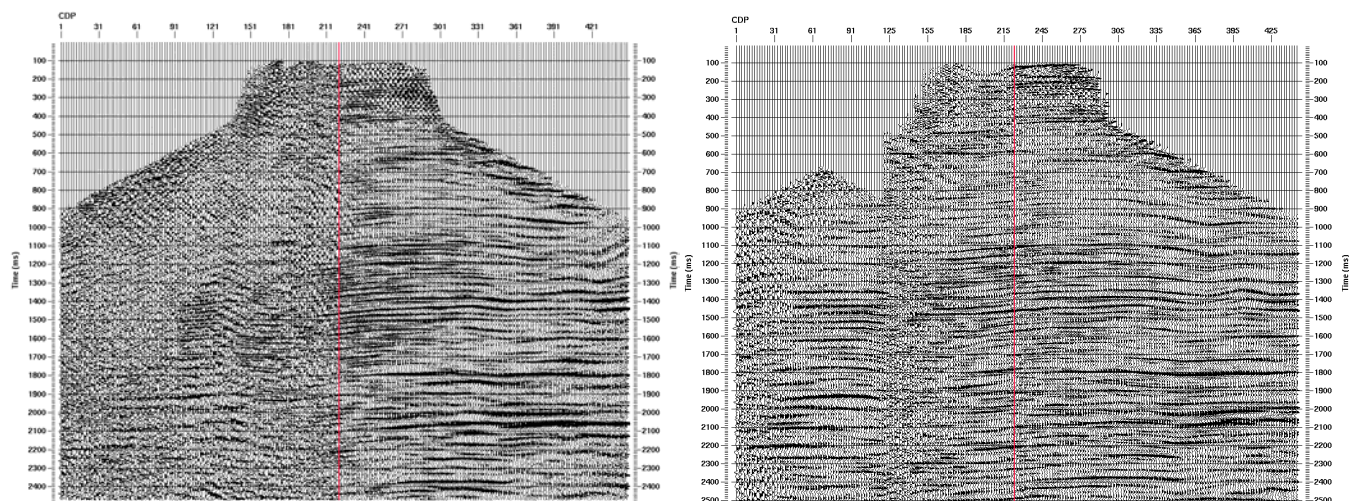
FIG. 4 Vertical component structure stack with f - x deconvolution for Vibroseis source (left) and dynamite source (right). A red line shows the approximate surface location of the transition zone.
