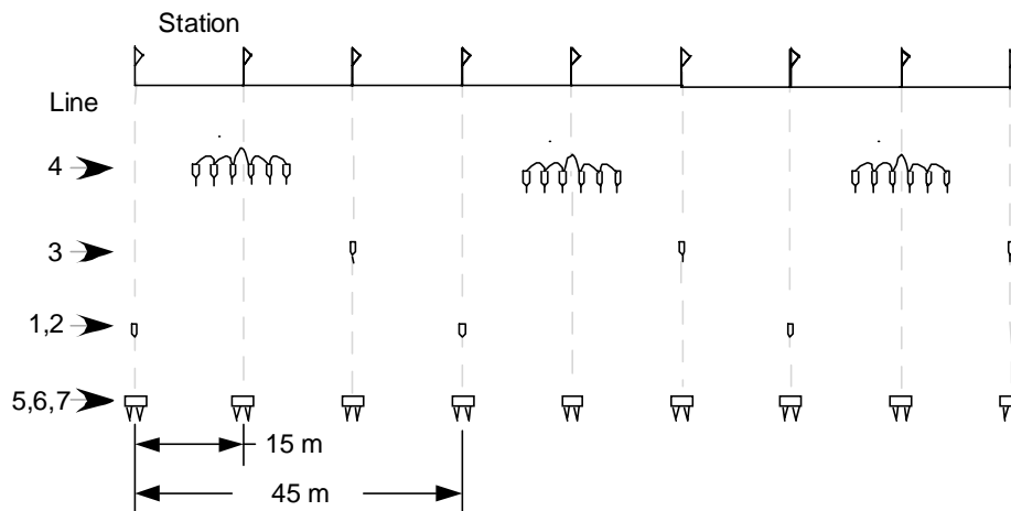
FIG. 2. Diagram of the receiver layout. Line 1: single Mark Products PE-44 hydrophones (under floating ice only). Line 2: single Oyo Geospace GS30CT marshphones, planted in sea floor/frozen ground below ice. Line 3: single marshphones in 0.30 m holes in ice. Line 4: six geophone arrays of marshphones, 2 m apart. Line 5: H1 component of Sensor 3-C geophones with SM-4 elements frozen into 0.15 m holes in the ice. Line 6: Vertical component. Line 7: H2 component.
