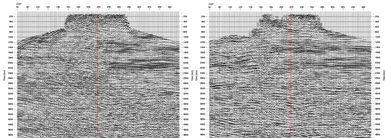
FIG. 5 Radial component structure stack with f - x deconvolution for Vibroseis source (left) and dynamite source (right). A red line shows the approximate surface location of the transition zone.
