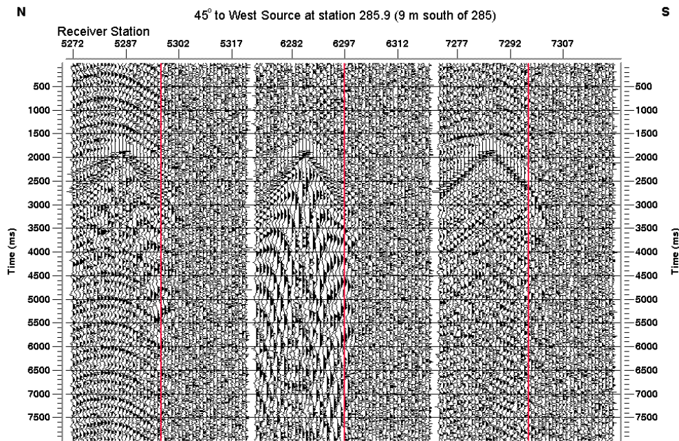
FIG. 3. Hammer source shot record, forty-five degree hit towards the west on the floating ice. H1(left), V(centre), and H2(right) components are shown. A red line shows the approximate surface location of the transition zone.
