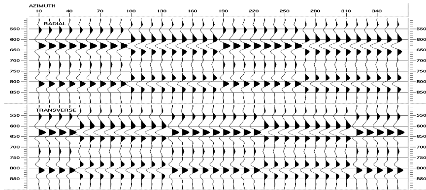
Figure 7: Limited-azimuth stacks that indicate a large amount of shear-wave splitting?
