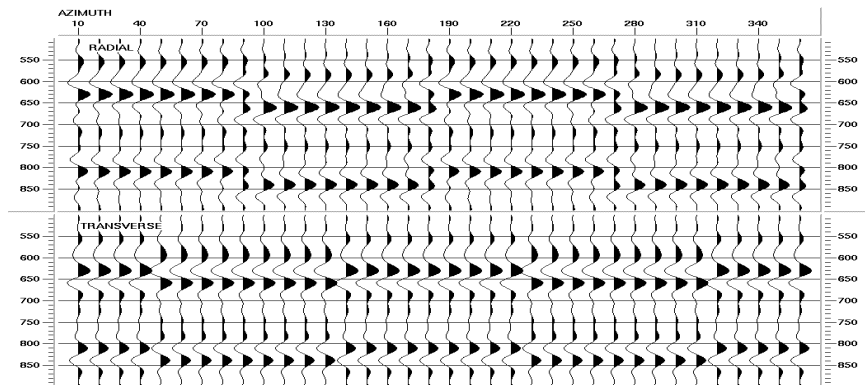
Figure 8: Limited-azimuth stacks for a single anisotropic layer with an S1 azimuth of 45° and a time delay of 30 ms.
