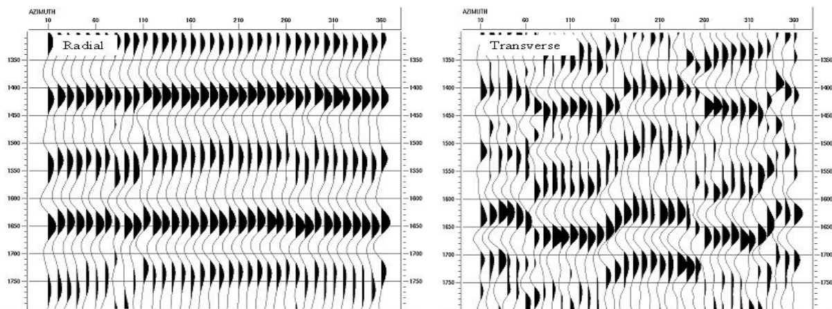
Figure 1: Horizontal-component limited-azimuth stacks from a 3-C/3-D dataset. Traces are stacked within 10° azimuth slices from 10° to 360°.
