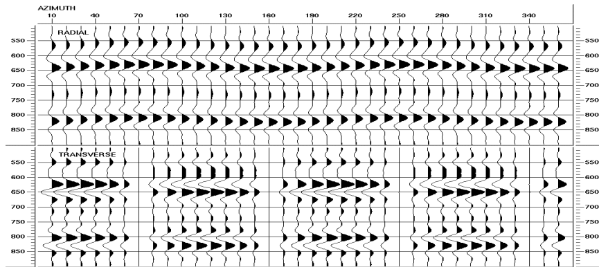
Figure 3: Limited-azimuth stacks for a single anisotropic layer. The S1 azimuth is 70° and S2 arrives 14 ms after S1.
