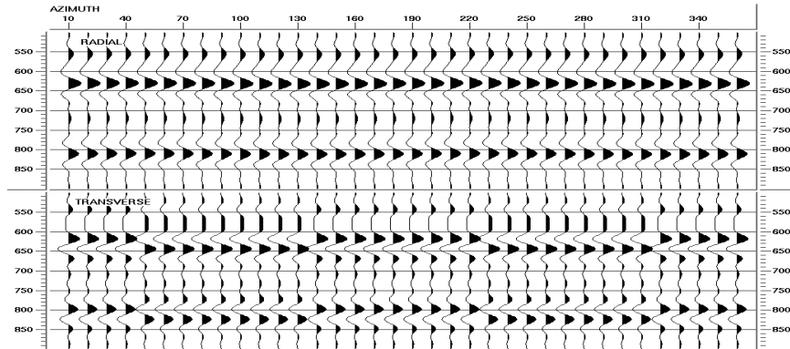
Figure 5: Limited-azimuth stacks for a single anisotropic layer with an S1 azimuth of 45° and time delay of 2 ms.
