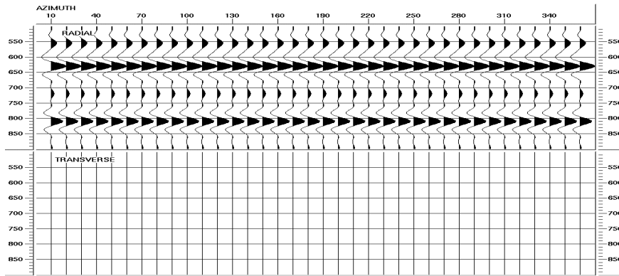
Figure 2: Synthetic limited-azimuth stacks of the radial (top) and transverse (bottom) components when no shear-wave splitting exists.
