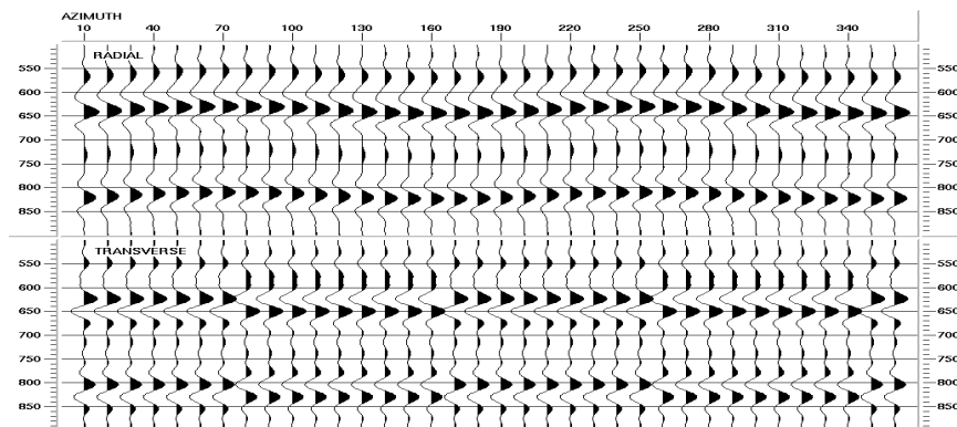
Figure 4: The same as Figure 2 except that each trace is scaled individually. Notice the abrupt polarity change in the transverse wavelet at the S1 and S2 azimuths, and the 90° phase difference between the radial and transverse wavelets.
