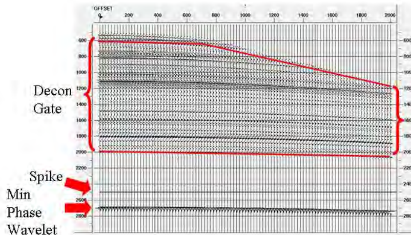
Figure 1. Synthetic seismograms (before addition of noise) used in the study. The spikes and wavelets at the bottom are used to monitor the effects of each step in the wavelet processing flow.
