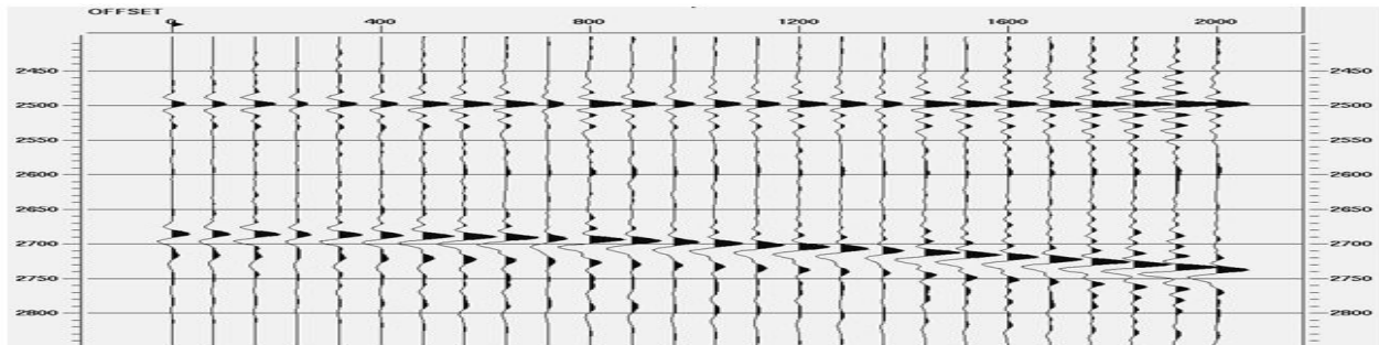
Figure 2: Deconvolution operators (top) and deconvolved wavelets (bottom) after surface-consistent deconvolution and spectral whitening when realistic noise is present. The phase is constant for all these traces, but the frequency content changes from trace to trace.
